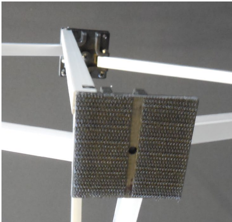
6. Secure fabric backer to Velcro tabs on frame.
